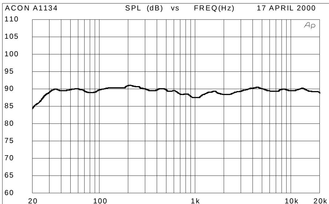
Obr. 9a: Active speaker ACON A1134 frequency response, 1m on axis in studio conditions
