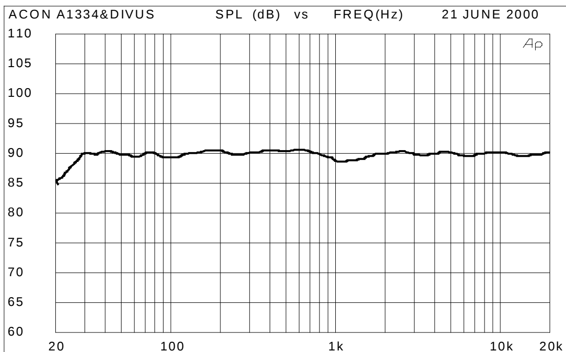
Obr. 9b: Active speaker ACON A1334/DIVUS frequency response, 1m on axis in studio conditions
